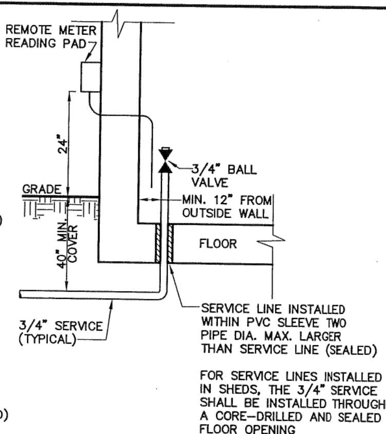
THROUGH FLOOR SERVICE
