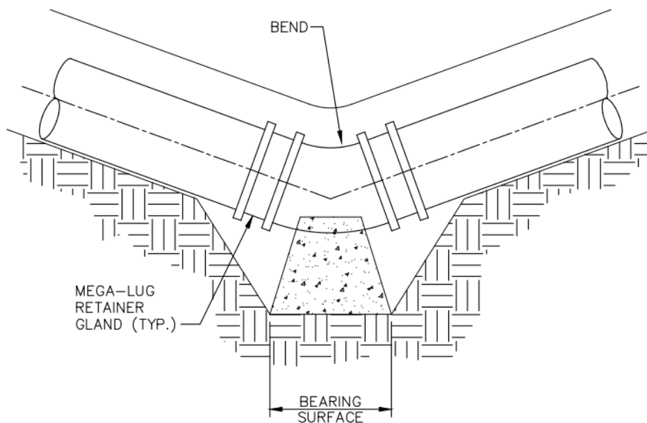
TYPICAL SECTION VERTICAL THRUST DOWNWARD NOT TO SCALE
