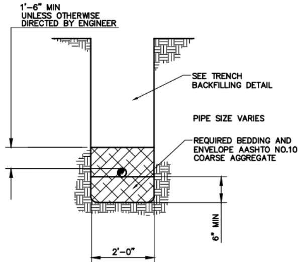
STANDARD PIPE BEDDING— WATER SERVICE NOT TO SCALE
