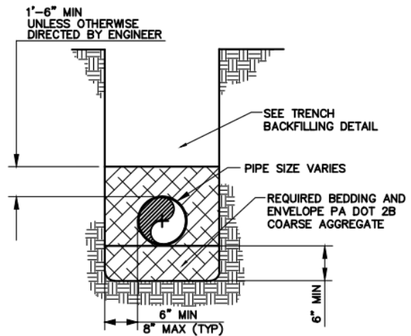
STANDARD PIPE BEDDING—SANITARY MAIN NOT TO SCALE
