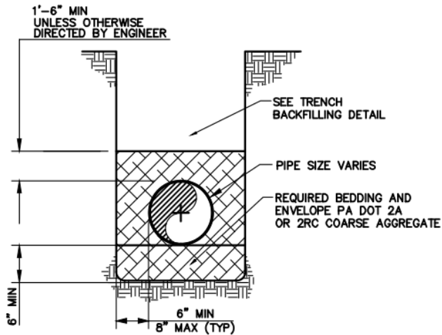
STANDARD PIPE BEDDING—WATER MAIN NOT TO SCALE
