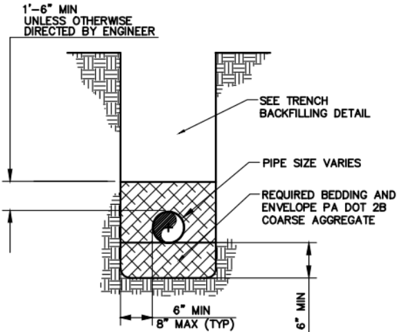
STANDARD PIPE BEDDING— SANITARY LATERAL NOT TO SCALE
