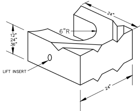
U-SHAPED COLLAR
