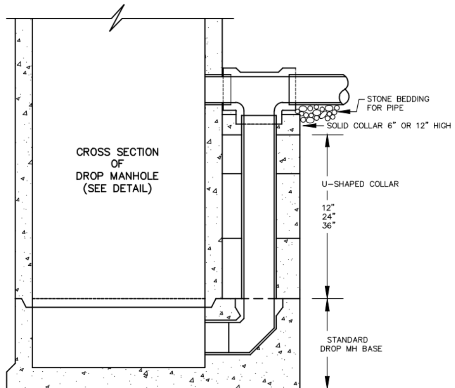
U-SHAPED COLLAR
