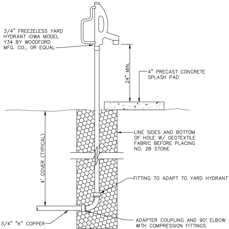
YARD HYDRANT DETAIL NOT TO SCALE
